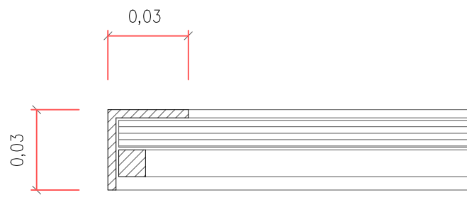
Corte Horizontal: escala 1/2
